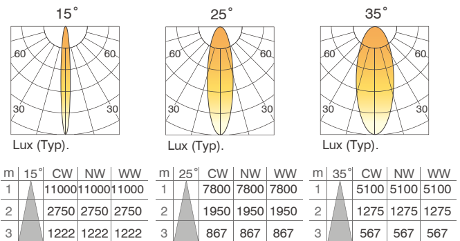
Light patterns of 24W AR111 Downlight for different angles.
