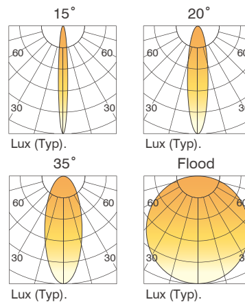
Light patterns of Glory series for different angles.
